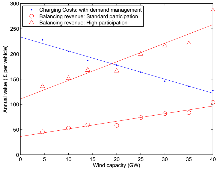
Figure 14: Comparison of the annual revenue generated through balancing and the average annual charging costs for a vehicle versus system wind power capacities between 4.6 GW and 40 GW. Linear fits are applied. Results are for a fixed participation of 1 million vehicles with V2G enabled.
