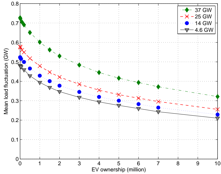
Figure 8: The mean 15 minute load fluctuation versus electric vehicle ownership for different UK wind power capacities.
