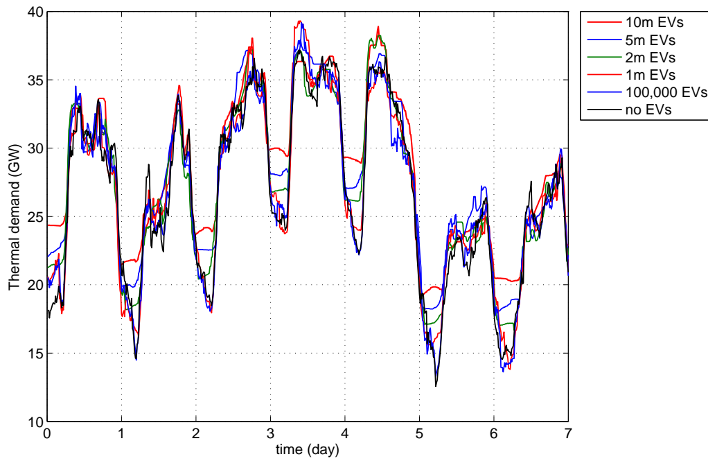
Figure 7: Comparison of load profiles featuring increasing numbers of electric vehicles stepwise up to 10 million vehicles, charging in a network with 14 GW of wind power capacity.
