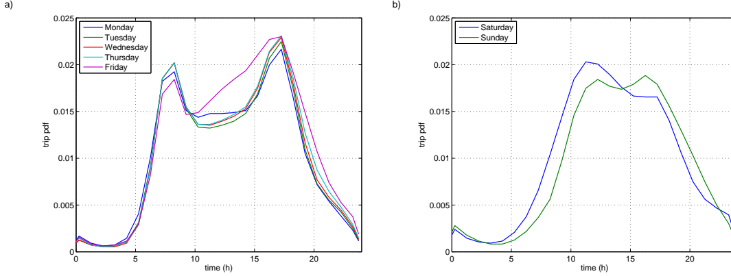
Figure 2: Trip density profiles used to generate the vehicle trips, separated into a) weekdays and b) the weekend.
