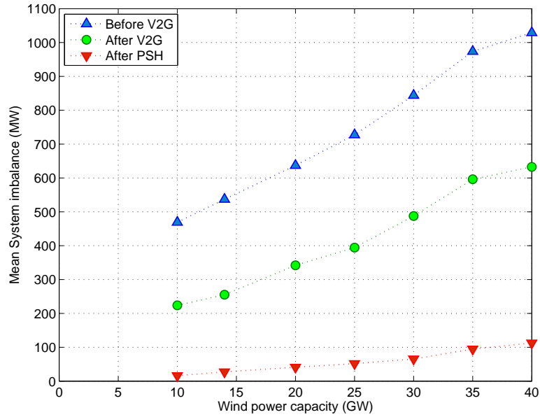
Figure 10: Average system imbalance against installed wind power capacity with a fleet of 1 million EVs, before and after vehicle charging and EV balancing, and the final imbalance after pumped storage hydro balancing.
