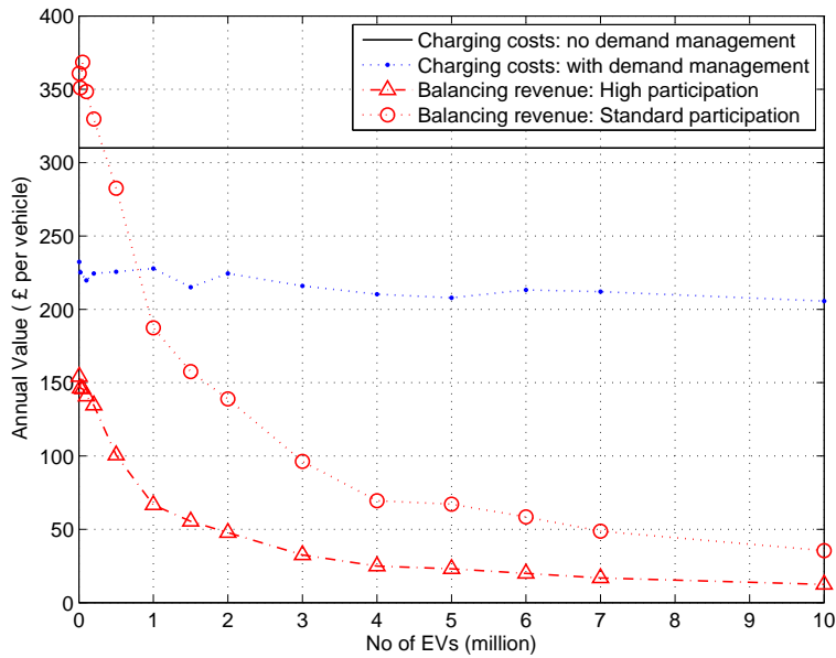
Figure 13: Comparison of the annual revenue generated through balancing and the average annual charging costs for a vehicle versus the number of EVs providing balancing services. Results from the 25GW wind power scenario.
