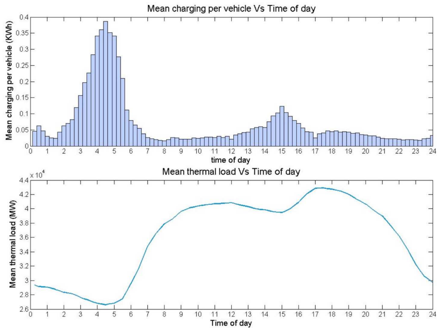
Figure 9: Comparison of the annual average charging distribution in 15 minute time bars divided by the number of EVs versus the average daily load profile with 4.6 GW of network wind power capacity.
