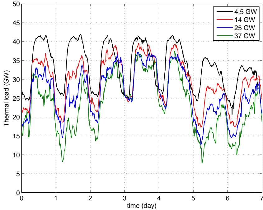
Figure 6: Thermal load without EV deployment for the four different wind generation scenarios.
