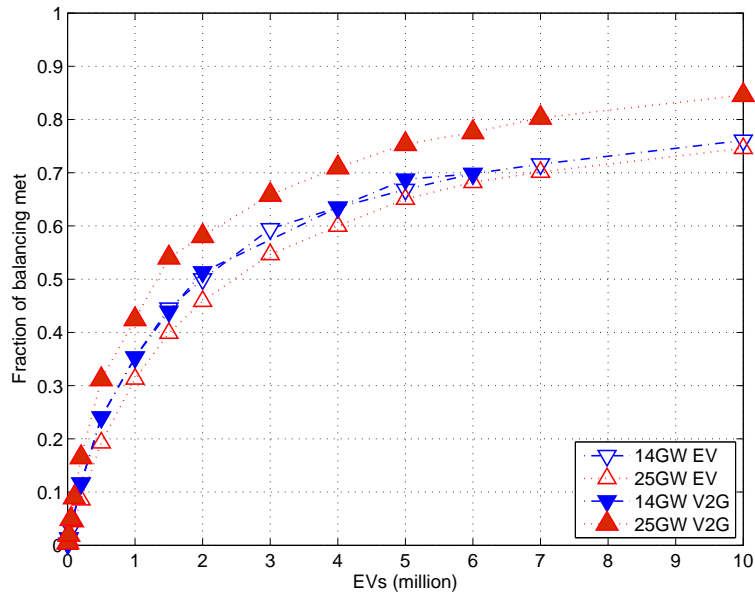
Figure 11: Comparison of the fraction of balancing met versus the number of EVs providing balancing services with V2G disabled (open symbols) or enabled (filled symbols) for installed wind capacities of 14 GW (downward triangles) and 25 GW (upward triangles), respectively.
