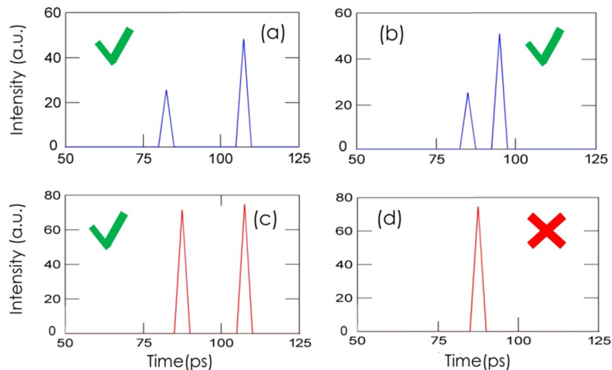
Figure 4. Comparison between the deconvolution's results obtained with a step size of 10 ps (a,b) and step size of 20 ps (c,d). For (a,c) the peak separation is 20 ps, whereas for (b,d) it is 10 ps. As it can be seen in (d), with 20-ps step size the algorithm is no longer able to distinguish peaks separated by 10 ps.
