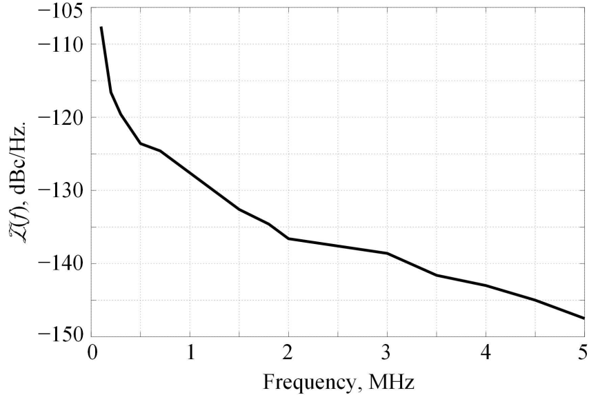
Fig. 8. Measured single sideband phase noise \mathcal{L}(f) of the phase conjugated 2444.69 MHz signal.
