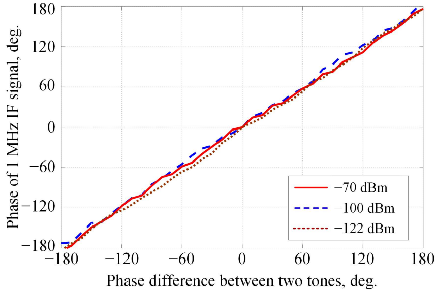
Fig. 11. Measured phases of the 1 MHz IF signals versus the phase differences between two tones for various input power levels in one receive chain.
