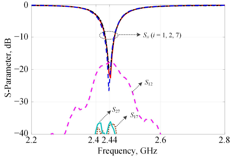
Fig. 5. Measured S -parameters of the 1 st , the 2 nd , and the 7 th elements in the fabricated 7-element array.
