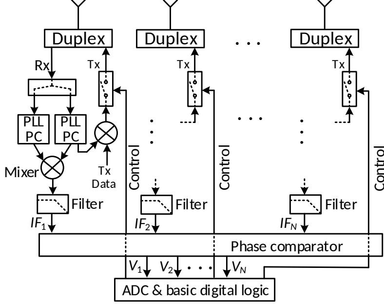
Fig. 2. Proposed dual-PLL PC RDA architecture.
