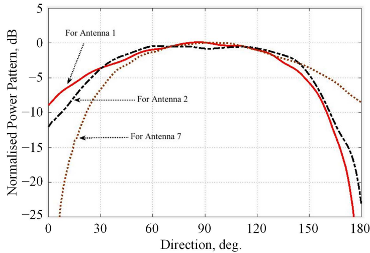
Fig. 6. Measured normalised active element patterns of the 1 st , the 2 nd , and the 7 th elements in the fabricated 7-element array. Boresight is along the direction \theta of 90°.
