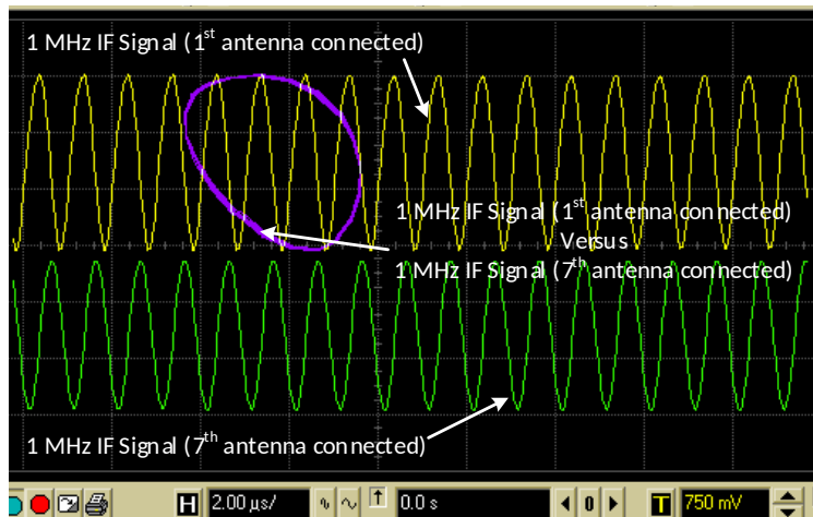
Fig. 10. Screen-shot of measured waveforms of 1 MHz IF signals when the 1 st and the 7 th antennas were connected. An Interference pilot at 2439.5 MHz was radiated along a spatial direction other than that of the 2FSK pilot.
