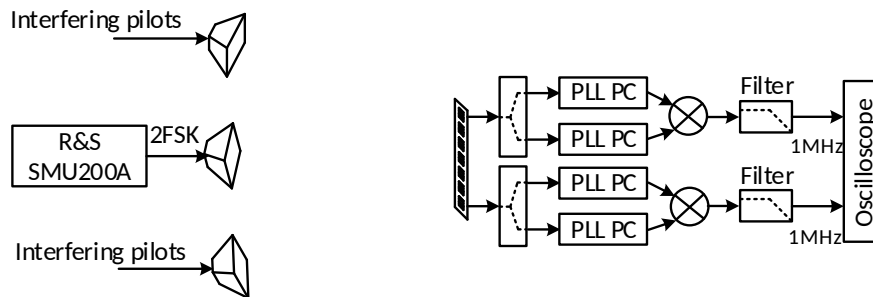
Fig. 7. Block diagram of the experimental setup.
