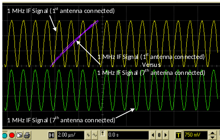
Fig. 9. Screen-shot of measured waveforms of 1 MHz IF signals when the 1 st and the 7 th antennas were connected. No interference pilots were radiated.
