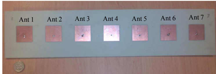
Fig. 4. Photo of fabricated 7-element 2.4 GHz patch antenna array.
