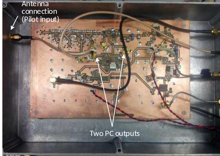
Fig. 3. Photo of fabricated frequency-tunable PLL PC.
