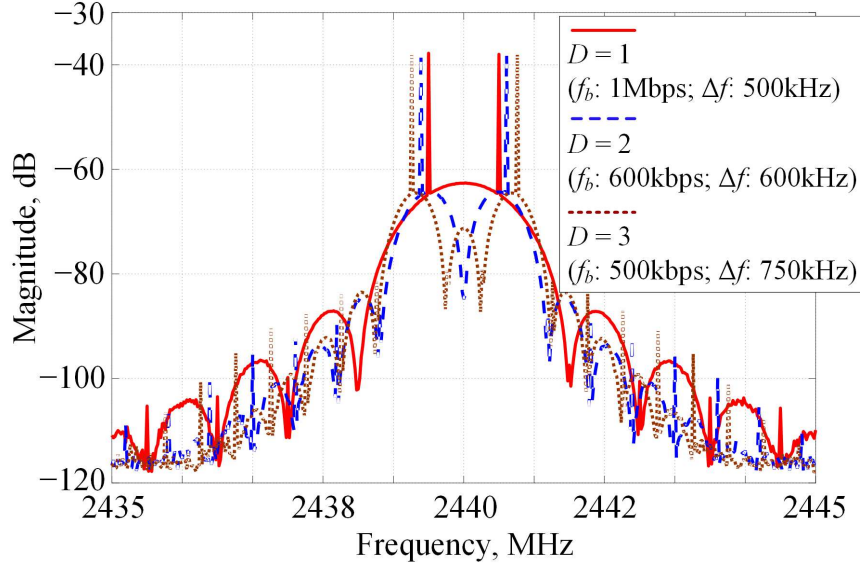
Fig. 1. Measured 2FSK frequency spectrum for D of 1, 2, and 3. f_c is fixed to 2440 MHz and f_b is the rate of PRBS data.
