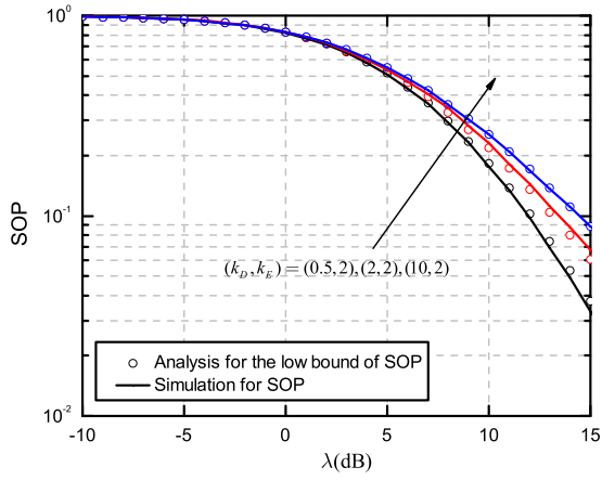
Fig. 2: SOP with changing (k_D, k_E) versus \lambda , (k_D, k_E) = \{(0.5, 2), (2, 2), (10, 2)\}
