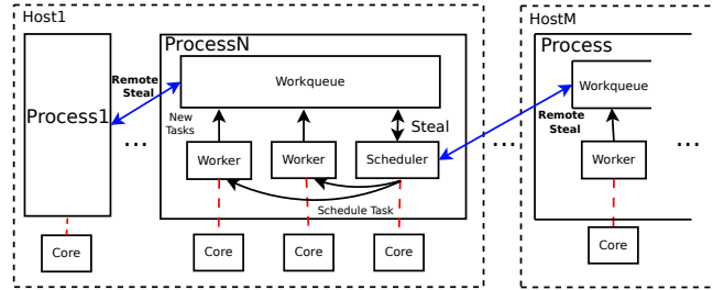
Figure 2: Framework Architecture for Distributed Task Parallelism
