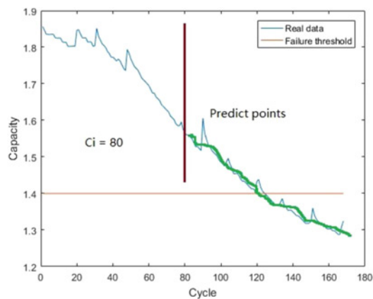
Fig. 3 RUL perdition curve for battery No. 5 at 80th cycle
