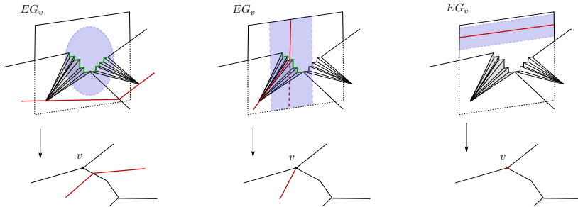
Figure 4.1. The three possible configurations, depending on the relative position of the hypergraph associated with W_i and the vertex v . In red: walls and hypergraphs. In green: K_i . In blue: C_i .
