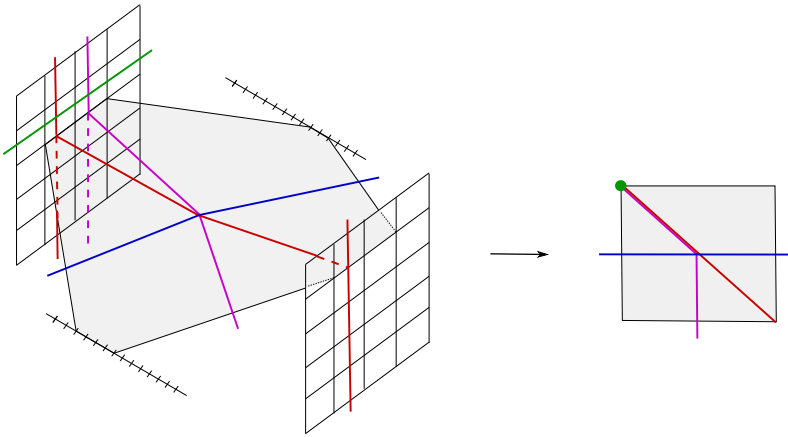
Figure 3.4. Examples of the three types of walls of \mathcal{E}G (left) and their associated hypergraphs in X (right), in the case A = \mathbb{Z}^2 , B = \mathbb{Z} . To avoid a busy picture, we only represent the case of a polygon of X with 4 sides. Blue: Walls/Hypergraphs associated with edges of X . Green: Walls/Hypergraphs associated with edges of \mathcal{E}G_{\text{bal}} of first type. Red and pink: Walls/Hypergraphs associated with edges of \mathcal{E}G_{\text{bal}} of second type.
