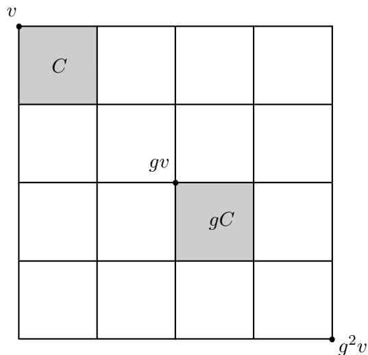
Figure 1: The 4 \times 4 grid K isometrically embedded in X , together with vertices v, gv and g^2v (black dots), as well as a square C and its translate gC (shaded).
