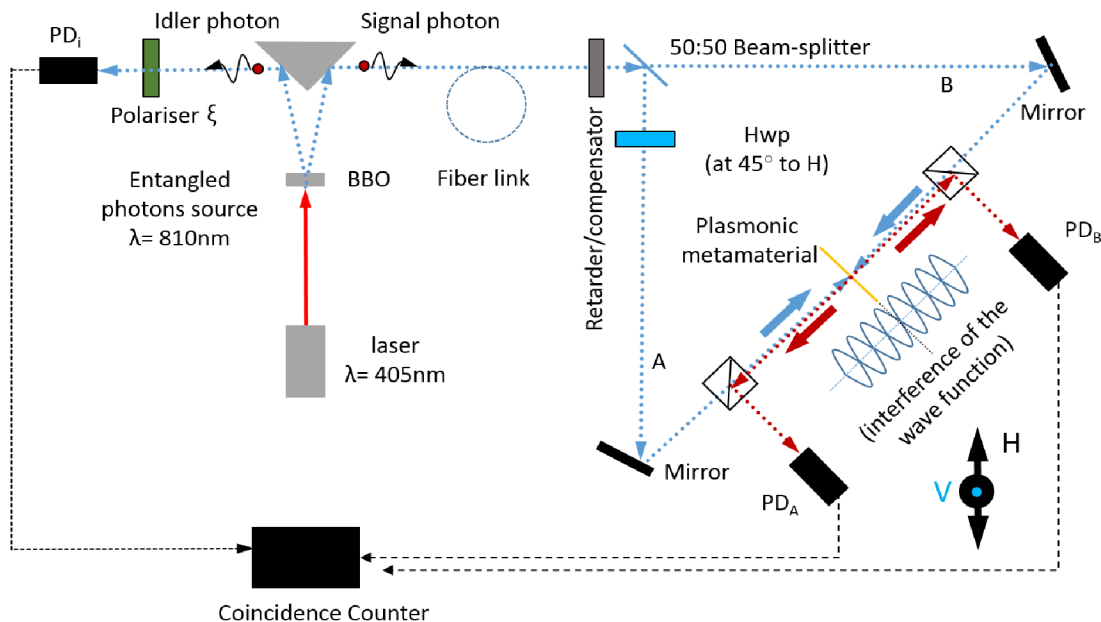
FIG. 1. Nonlocal dissipation management with entangled photons. Polarization-entangled photon pairs are generated by a type II spontaneous parametric down conversion process (laser at 405 nm impinging a BBO nonlinear crystal). One photon of the pair is introduced in the interferometer (the signal photon at the 50/50 beamsplitter) and can take two paths (A and B) with a fiber link and a compensator for synchronization issues. Hwp is a half waveplate in arm A. A thin metamaterial plasmonic absorber is introduced in the polarization-sensitive interferometer. By detecting the idler photon outside the interferometer with the help of a polarizer ( \xi ), one can non-locally prevent or allow deterministic absorption of the signal entangled photon that dissipates through coupling into a plasmon of the absorber placed in the interferometer. PD_A , PD_B and PD_i are photon detectors.
