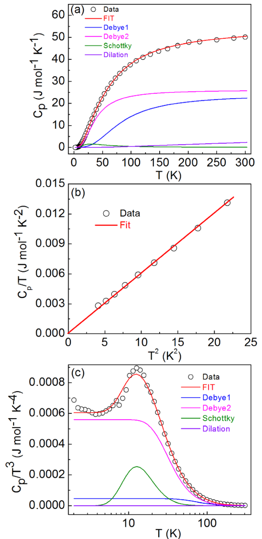
FIG. 2. (a) Fit to the temperature dependence of the heat capacity ( C_p ) of SnSe using two Debye terms (blue and pink line), Schottky mode (green line) and lattice dilation (purple line). (b) C_p/T versus T^2 illustrating the absence of a significant electronic contribution to C_p . (c) C_p/T^3 versus T , highlighting the Schottky contribution at low temperatures.
