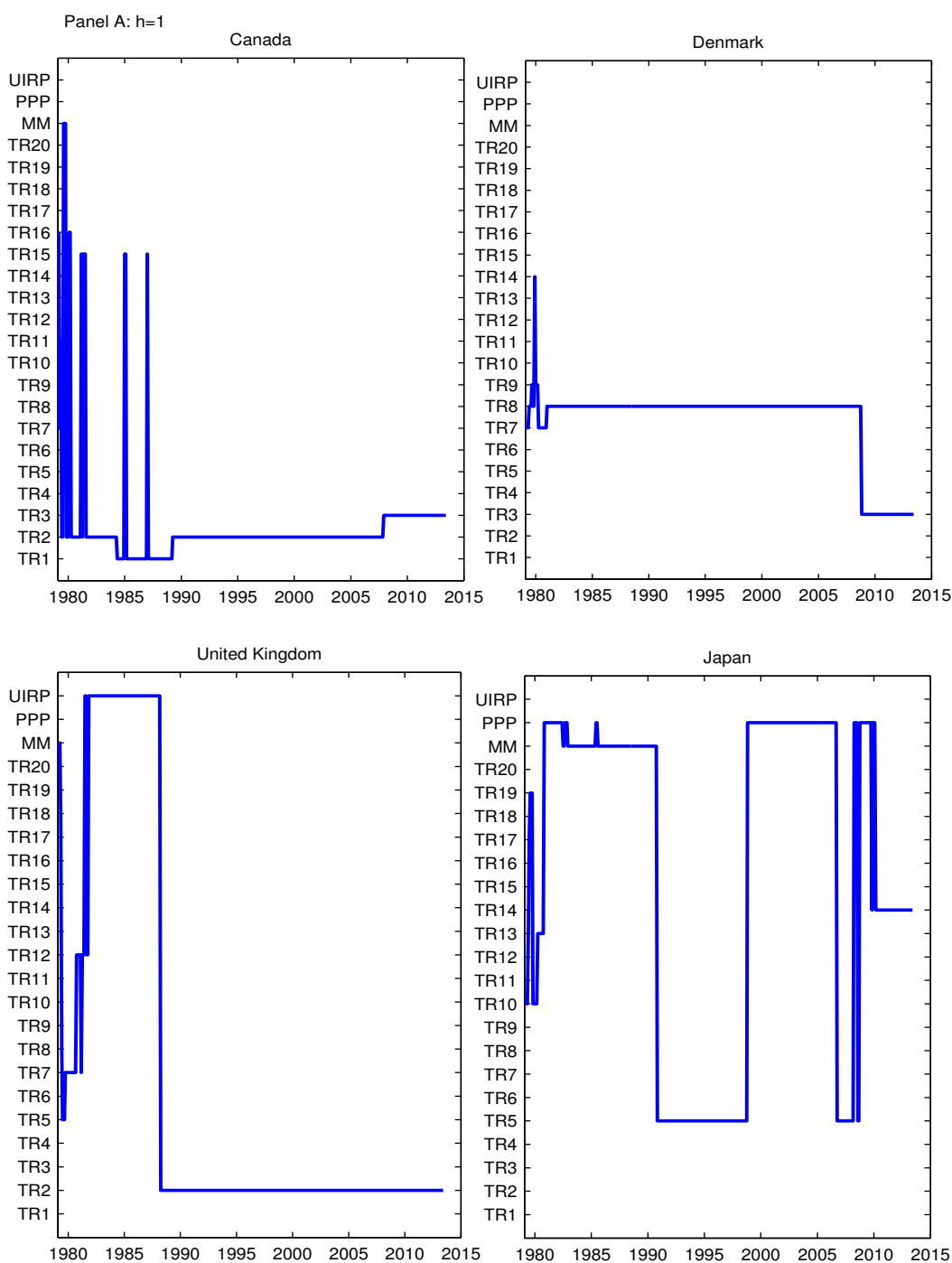
Figure 5: Predictors with the Largest Posterior Probability at Each Period
