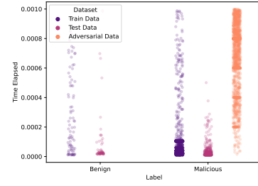
Figure 5: Expansion of related feature, TimeElapsed .
