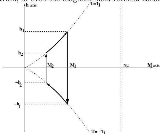
FIG. 1. ‘Carnot’ cycle for a heat pump using negative temperatures. The area enclosed by the loop equals the total energy transferred per cycle. For the nuclear spin system the equation of the temperature- T isotherm is h = (kT/\mu)\text{arc tanh}(M/N\mu) . The vertical line at M = N\mu is an asymptote of all the isotherms, both for positive and negative temperatures.
