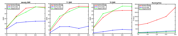
Fig. 1: Reconstruction performance as a function of L
