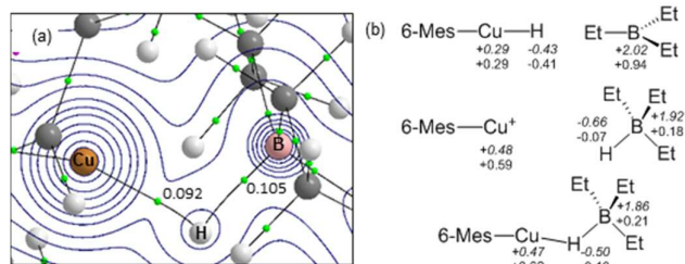
Figure 3. (a) Detail of the QTAIM molecular graph of 5 showing electron density contours in the \{\text{Cu}/\text{H}/\text{B}\} plane. Bond critical points (BCPs) are shown as green spheres and key values of \rho(r) (the associated BCP electron densities) are indicated in au. (b) Computed atomic charges for 5 and selected comparator species (QTAIM charges in italics; NBO charges in plain text). Full QTAIM metrics are provided in the ESI, along with equivalent \rho(r) values obtained with a range of different functionals..
