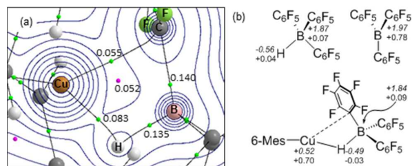
Figure 4. (a) Detail of the QTAIM molecular graph for 6 showing electron density contours for the (Cu/H/B plane). Bond critical points (BCPs) and ring critical points (RCPs) are shown as green and magenta spheres respectively and \rho(r) values of key CPs are indicated in au. (b) Computed atomic charges for 6 and selected comparator species (QTAIM charges in italics; NBO charges in plain text). Full QTAIM metrics are provided in the ESI along with equivalent \rho(r) values obtained with a range of different functionals.
