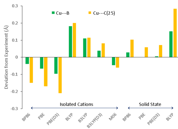
Figure 5. Cu \cdots B and Cu \cdots C(25) distances in 5 computed with various functionals and displayed as deviations from the experimental values of 2.283(3) Å and 2.619(3) Å respectively. Calculations employed either the isolated molecule (Gaussian) or the extended solid state via periodic boundary conditions (CP2K).
