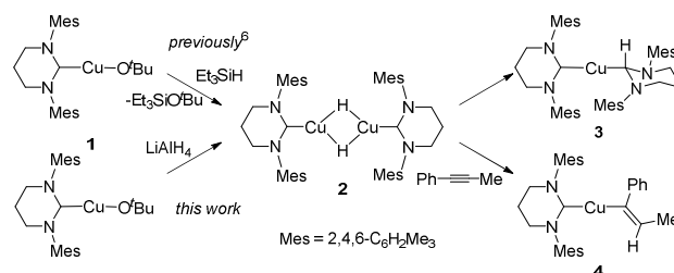
Scheme 2. Synthesis and reactivity of [(6Mes)Cu(μ-H)] 2 ( 2 ).
