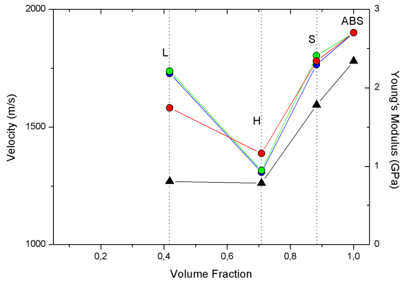
Fig. 4. Volume fraction vs Velocity as a function of axial orientation and Young's modulus. Blue circles: along x axis; Green circles: along y axis; Red circles: along z axis; Black triangles: Young's Modulus.
