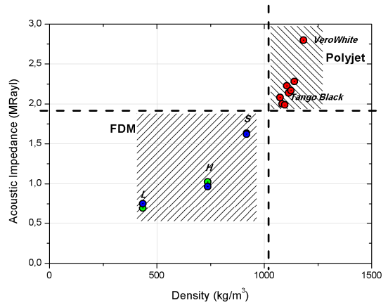
Fig. 5. Variation of acoustic impedance with density. Green circles: acoustic impedance of FDM cubes along build direction; Blue circles: acoustic impedance of FDM cubes normal to build direction; Red circles: acoustic impedance in thickness direction of Polyjet samples with different content of Tango Black/VeroWhite.
