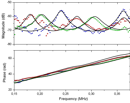
Fig. 2. Magnitude and phase spectra of the transmission coefficient of Polyjet samples. Blue circles : 100% VeroWhite; Red triangles : 100% Tango Black; Green squares : Sample 7 49.65% Tango Black. Solid lines : correspond to acoustic model fitting considering the whole sample as a homogeneous plate.
