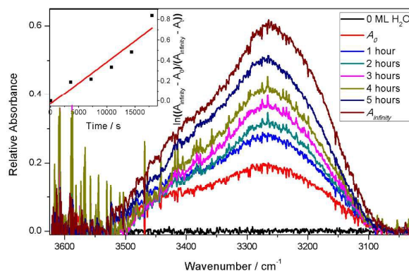
Figure 1: Time-resolved RAIR spectra of the νOH stretch region of 0.5 ML H 2 O on aSiO 2 at 18 K. The time between each RAIR spectrum was one hour as this was determined to be the average time between scans when H 2 O is annealed at the other temperatures investigated. The sharp peaks are due to gas-phase H 2 O in the optics boxes on the air side of the UHV apparatus. Inset is the kinetic analysis using eqn 1. Figure also found in reference [19].
