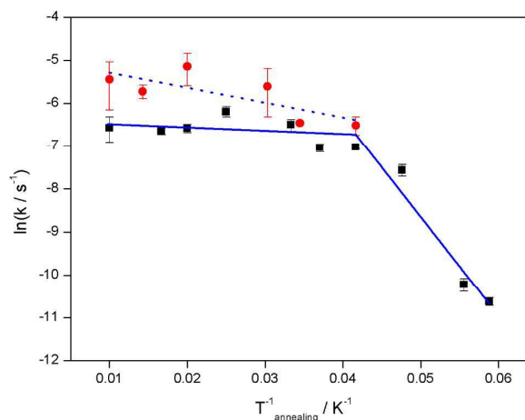
Figure 2: Arrhenius analysis of the kinetics of \text{H}_2\text{O} agglomeration on \text{aSiO}_2 (filled squares) and HOPG (filled circles) with lines representing the best linear fit for the two surfaces along with error bars. The solid lines represent the fits to the two \text{H}_2\text{O} on \text{aSiO}_2 regions as discussed in the text.
