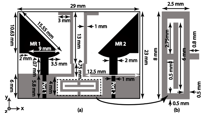
Fig. 1: Geometry of the proposed UWB MIMO antenna system. (a) Layout with dimensions and (b) CSRR unit with dimensions.
