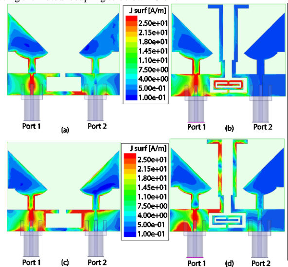
Fig. 4: Surface current distribution with and without CSRR and Stubs. (a,b) at 3.45 GHz and (c,d) at 6 GHz. Only port 1 is excited. The plot illustrates how the stubs and CSRR resonator reduce the coupling between the two elements. Notice that in (Figs. 4b and d) there is very little current on the second (right) antenna from port-1 when the stubs and the CSRR have been introduced.
