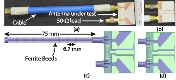
Fig. 5: Photo of the developed prototype with the short feeding cable used in the simulation and measurements (a) top side of fabricated prototype and (b) bottom side of fabricated prototype and (c) simulated model in HFSS with short feeding cable and (d) simulated model in HFSS without cable.
