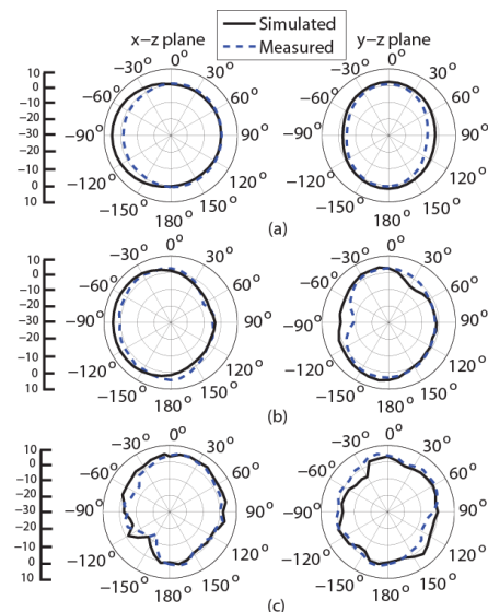
Fig. 7: Simulated and measured radiation pattern (a) 3.5 GHz and (b) 7 GHz and (c) 10.5 GHz, exhibiting near-omnidirectional radiation suitable for UWB-MIMO systems.
