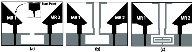
Fig. 2: Geometry of the proposed UWB/MIMO with ground variations. (a) Without CSRR and stubs (b) with two stubs and (c) with CSRR and stubs.
