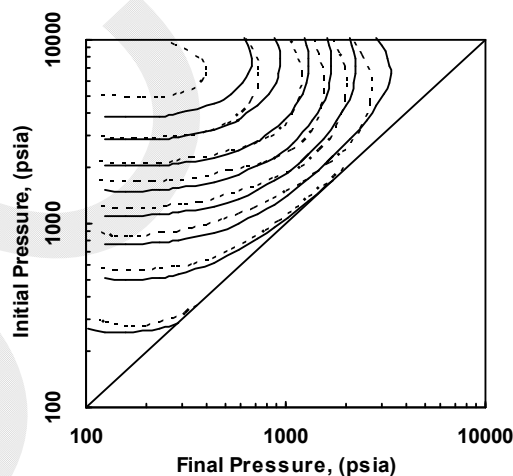
Fig. 4. Katz diagrams, dashed lines, for allowable pressure drop in a throttle valve in comparison with this work, solid lines, for 0.7 gas gravity, Temperatures are respectively from top to bottom: 184, 170, 150, 130, 110, 90, 70, 50 °F. Gas compositions are: y_{c1}=0.8605 , y_{c2}=0.0606 , y_{c3}=0.0339 , y_{ic4}=0.0084 , y_{nc4}=0.0136 , y_{nc5}=0.023 .
