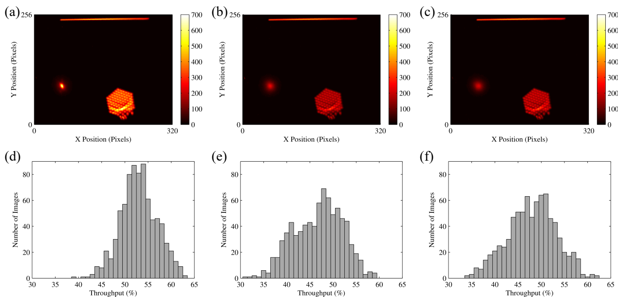
Figure 3. Colour map images of the camera sensor for averaged, reduced data showing the output of the hybrid reformatter (along the very top), the secondary lantern (lower right) and the telescope PSF (lower left) from the reference path for (a) closed-loop, (b) tip-tilt only and (c) open-loop modes of AO correction. Note: The camera has 30\,\mu\text{m} pixels and the secondary lantern output is distorted due to an imperfect cleave. Bottom row: Histogram plots showing percentage transmission distribution over the number of images acquired for (d) closed-loop, (e) tip-tilt and (f) open-loop AO modes. Hot pixel removal and background correction algorithms have been applied prior to evaluating the transmission for each image frame acquired.
