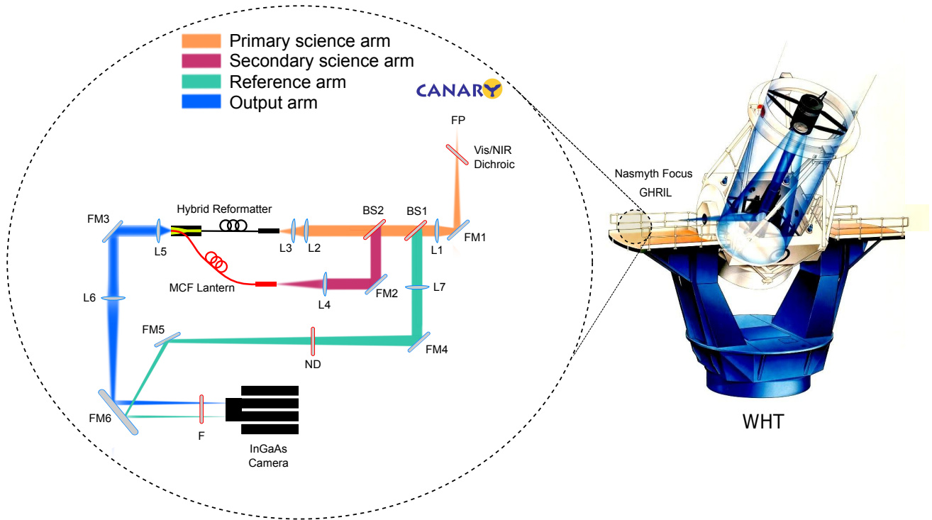
Figure 2. Schematic diagram showing the free-space optical setup used for the on-sky tests. Stellar light collected by the William Herschel Telescope is fed through the CANARY AO system which generates a corrected multimode PSF. A dichroic is used to remove the visible part of the spectrum ( < 1000 nm) from the light beam, which is then collimated using a lens (L1). Using a beamsplitter (BS1), 10 per cent of the collimated beam is fed to a reference path containing a 0.6 absorptive neutral density filter (ND), and re-imaged the PSF onto the camera using L7. The remaining light passes through another beamsplitter (BS2), which reflects 81 per cent to the secondary science arm. The light in this arm is focussed by L4 and allows the core of the PSF to be imaged onto the multimode port of the secondary lantern. The rest of the light is focussed by L2 and L3 onto the hybrid reformatter which samples the whole PSF. The reformatted output from both the hybrid reformatter and secondary MCF lantern are imaged onto the camera using lenses L5 and L6. The fold mirrors (FM1 - FM6) are utilised for beam steering. An H -band spectral filter (F) was placed at the entrance to the camera. (WHT image courtesy of the Isaac Newton Group of Telescopes, La Palma).
