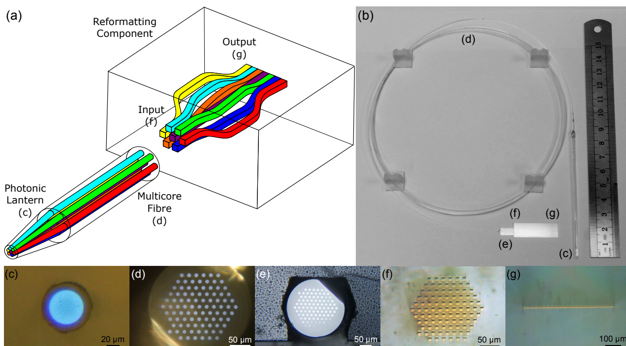
Figure 1. (a) 3-D schematic of a simplified 7 - core hybrid reformatter. The colours differentiate different waveguide paths. (b) Photograph of the hybrid reformatter device. (c) Photonic lantern with multimode input port. (d) Facet of the multicore fibre, with the extra 92 nd core visible in the bottom left. (e) Multicore fibre placed in a custom ULI fabricated V-groove. (f) Input facet of the ULI manufactured reformatting component. (g) Pseudo-slit output of the reformatting component.
