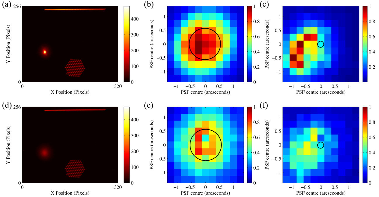
Figure 4. Dither plots for the night of 2014 October 12. Top row shows closed-loop operation, and bottom row tip-tilt operation. Left column shows averaged reduced data obtained from the camera. Middle column images show the position of the dithered PSF, with the colour bar being normalised flux for the slit of the hybrid reformatter. The right column images show the position of the dithered PSF, with the colour bar being normalised flux for the secondary photonic lantern. The black circles represent the angular size of the input fibre in each science arm
