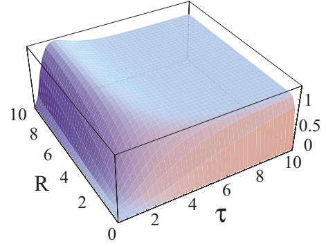
FIG. 2. (Color online) Plot of the quantity D_{a=0}(R, \tau) as a function of \tau = \gamma t and R .
