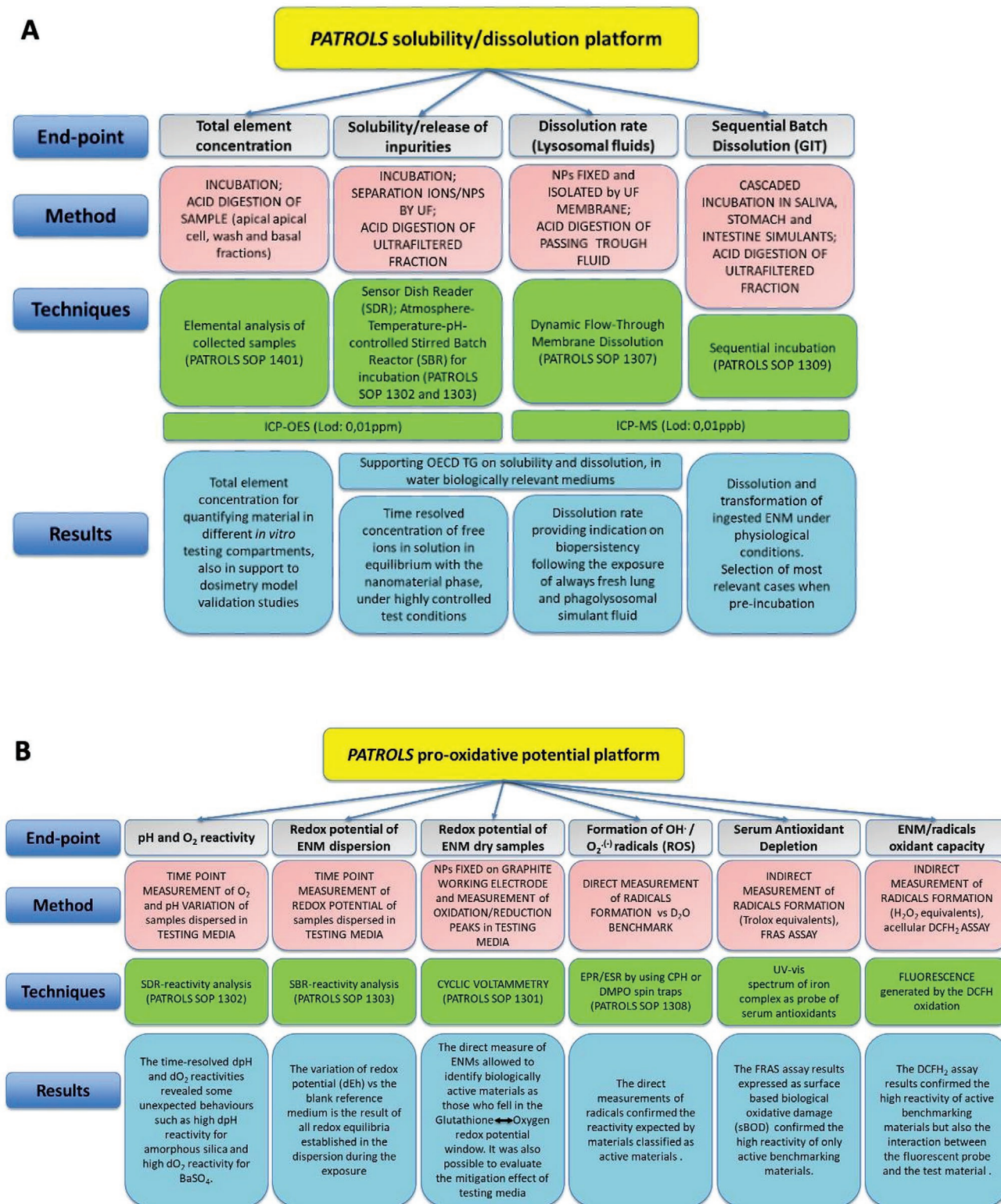
Figure 3. The PATROLS physicochemical testing strategy detailing the endpoint for evaluation, the corresponding methods applied, and the corresponding results and outputs. A) PATROLS dissolution multi-method platform; [22,37] B) PATROLS pro-oxidative multi-method platform.
