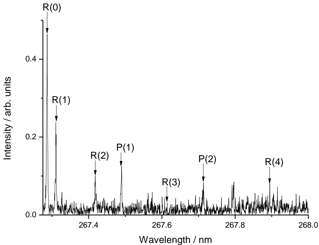
Figure 1: 3+1 REMPI spectrum of the B'-X(0,0) band of D 2 , with labels indicating the assigned transitions.
