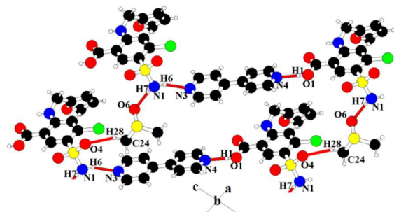
Fig. 2 Two-dimensional hydrogen-bonding network observed in co-crystal ( 2 ), viewed along [010].
