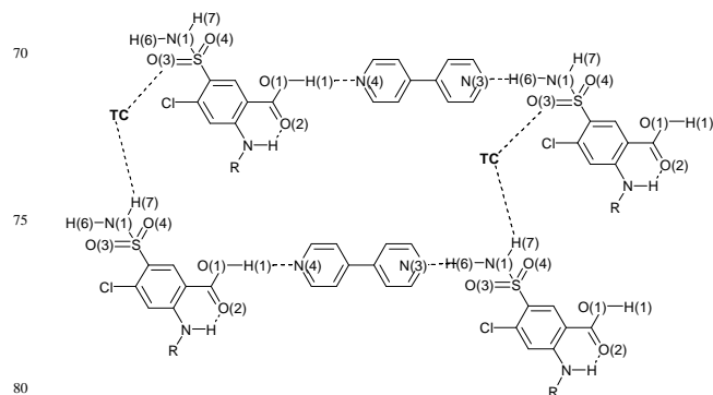
Scheme 1: Schematic illustration of the two-dimensional network observed in all ternary co-crystals. R=furfuryl, TC=ternary component (DMF; DMSO; MeOH; ethanol; 2-propanol; 1-butanol; ethylene glycol; 1,4-butanediol; hydroquinone). The dotted lines indicate hydrogen bonding interactions.
