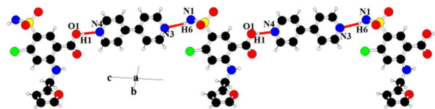
Fig. 3 Columnar arrangement between furosemide and bipyridyl common to all ternary co-crystals ( 2 )–( 10 ), viewed along [100].
