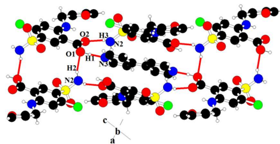
Fig. 1 Packing arrangement in co-crystal (1) viewed along [010].
