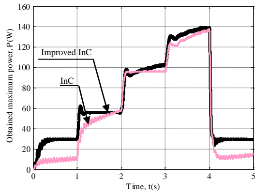
Fig. 10. Obtained maximum output power with the InC and improved InC algorithms under both the variations of the solar irradiation and temperature
