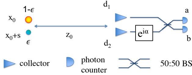
Figure 2. Schematic of two sources with a separation of s in the object plane, with relative intensities \epsilon and 1 - \epsilon , at a distance z_0 from the collectors. Two collectors at d_1 and d_2 direct light into a two-input interferometer consisting of a phase shift of \alpha and a 50:50 beam splitter, followed by photon counters. A collector can be any optical element that collects light. This could incorporate lenses or in the case of this experiment, two fibre connectors that present only the bare fibre core diameters in the direction of the source.
