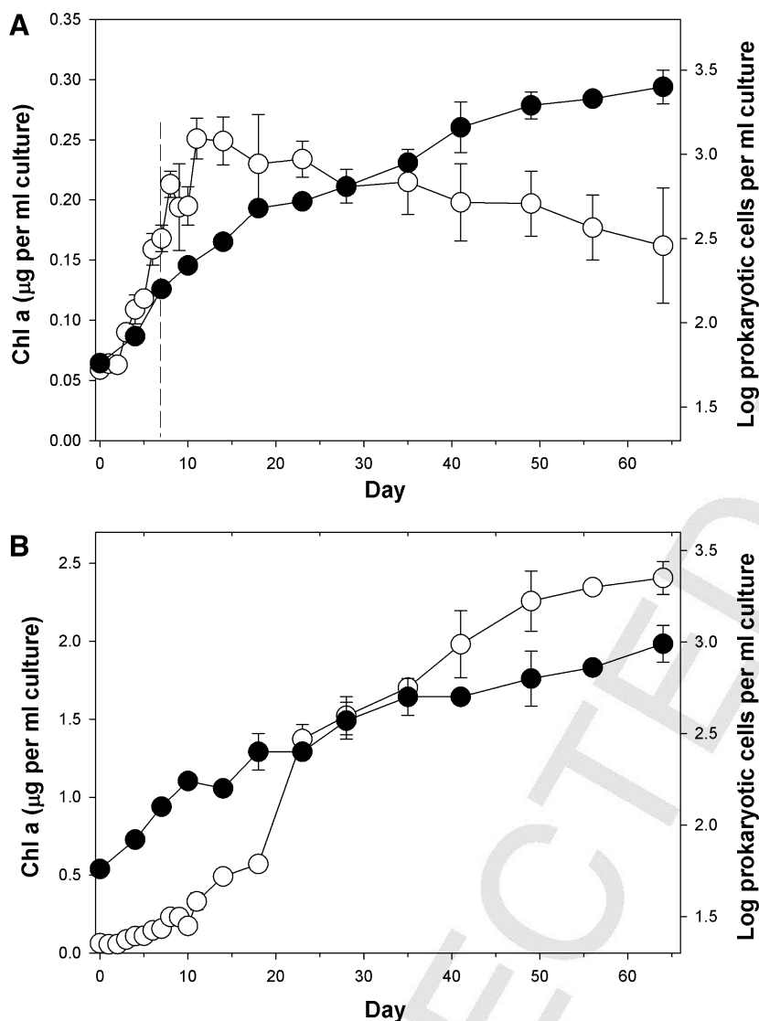
Fig. 1. Chlorophyll a concentrations (open circles) and prokaryotic (bacterial and archaeal) cell numbers (solid circles) in incubations of non-axenic S. costatum strain CCAP1077/1C amended with (A) or without (B) ANS crude oil – respectively flasks O1-3 and C4-6. The hatched line at day 7 (top panel) indicates the time point the oil was added. Note difference in scale of the left-hand y-axis in the two plots. Some error bars are smaller than the symbol.
