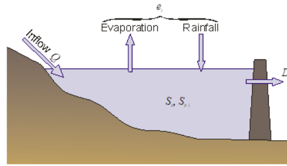
Figure 1: Schematic of the components of the reservoir water balance equation.
