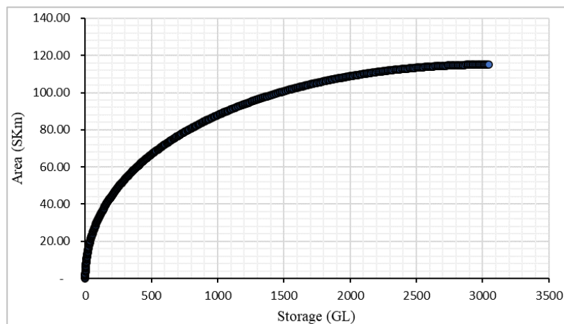
Figure 3: Storage-Area Relationship for Lake Hume. Data obtained from (Lehner et al., 2011)
